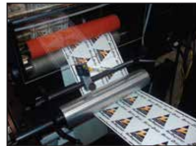
Adjustable sensor electronically sends web corrections to the servo-drives.
