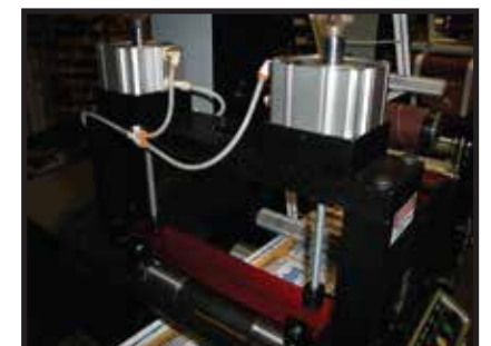
Pneumatic Die Release to Prevent Die Damage
